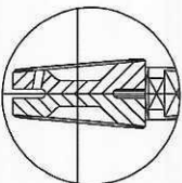
Flexible Wedge
